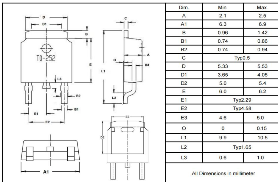
TO-252
